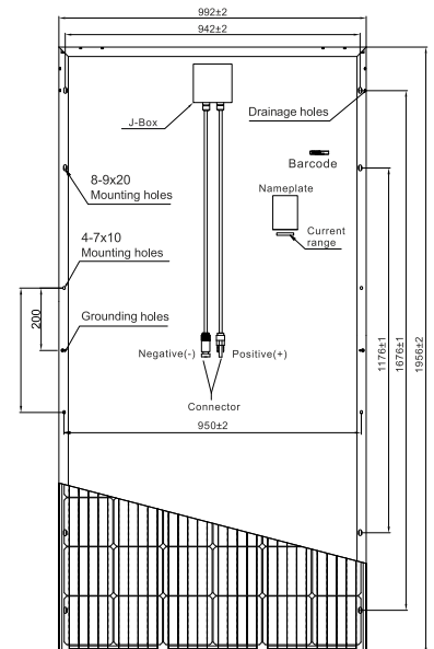
Dimensions of PV Module Unit: mm
